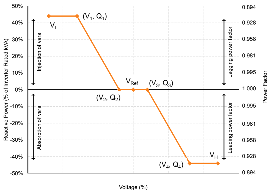
Figure 6-1: Voltage-VAR Characteristics
