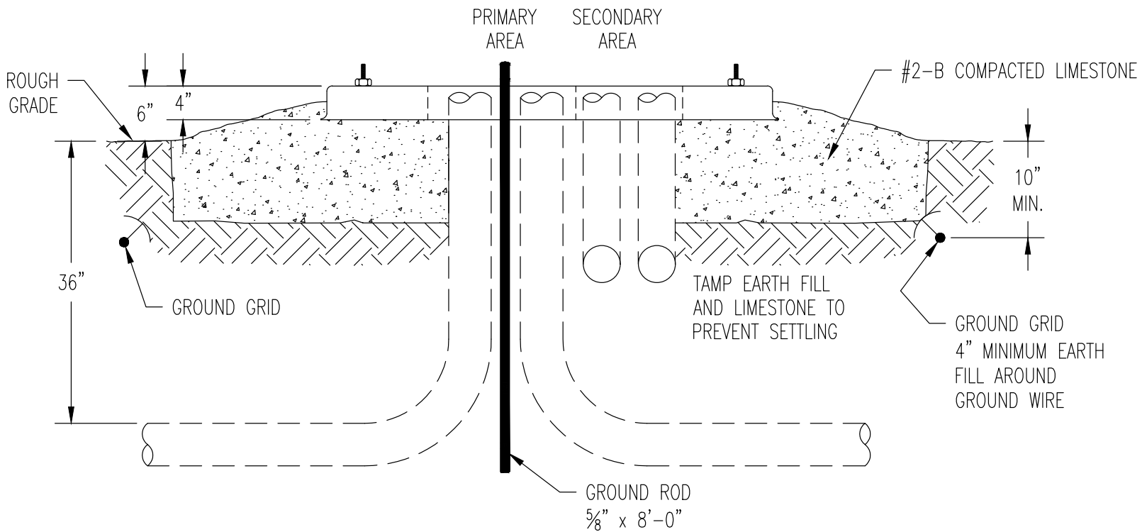
1-PHASE TRANSFORMER PAD DETAILS (SIDE VIEW)
