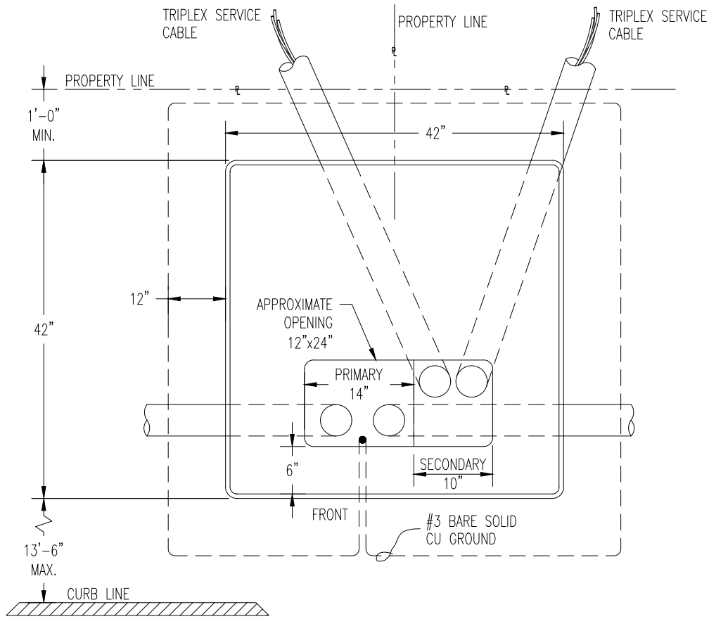
1-PHASE TRANSFORMER PAD DETAILS (TOP VIEW)
