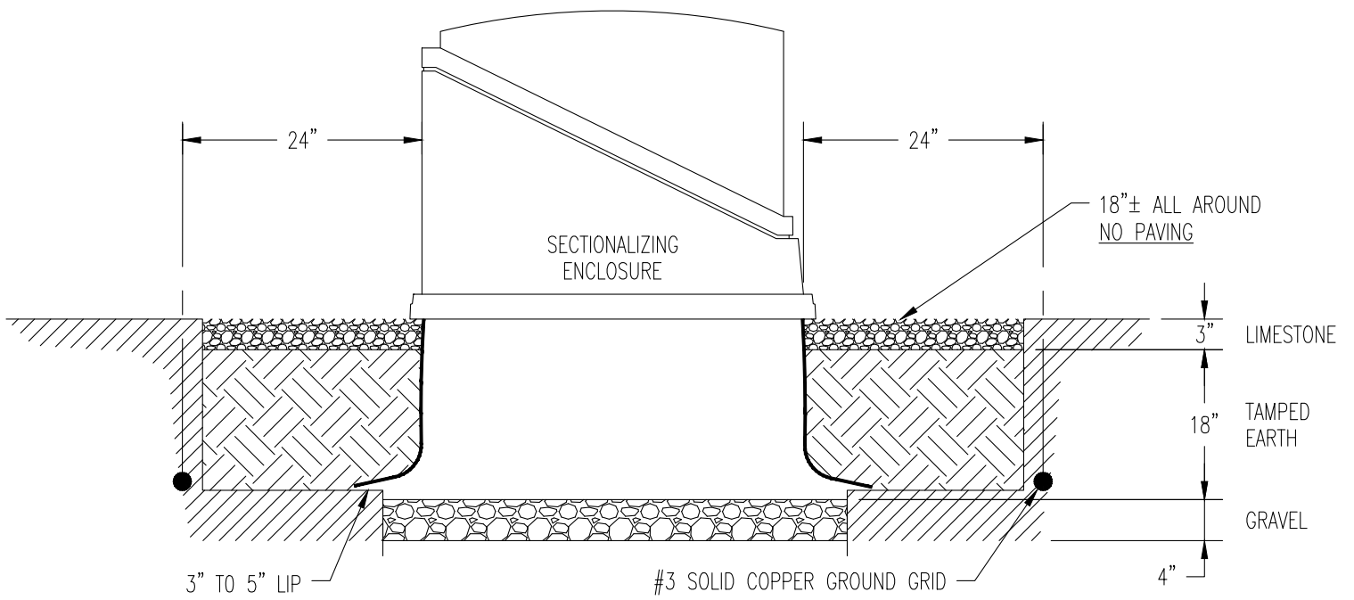
SECTIONALIZING ENCLOSURE PROFILE
