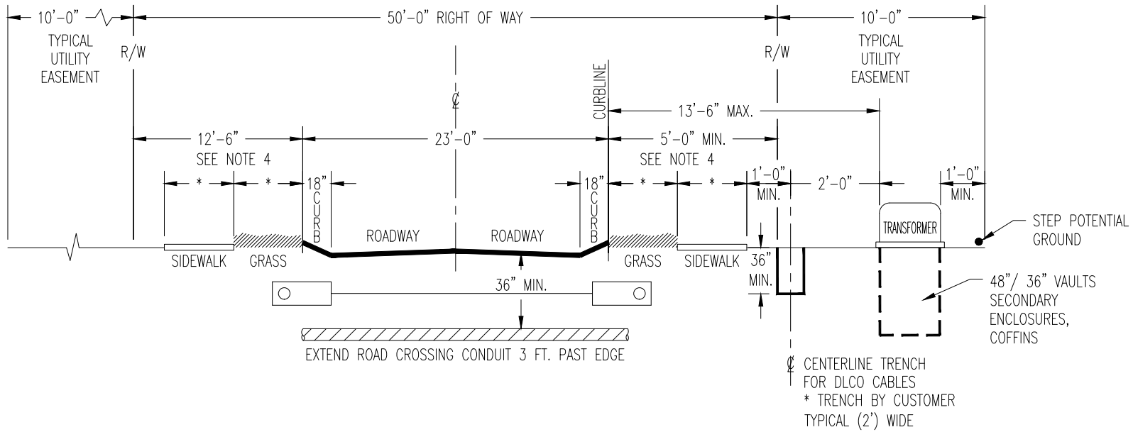
TYPICAL ROAD PROFILE
